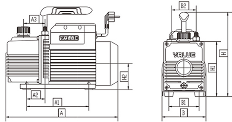
The dimension for VEN series pump(unit:mm)
